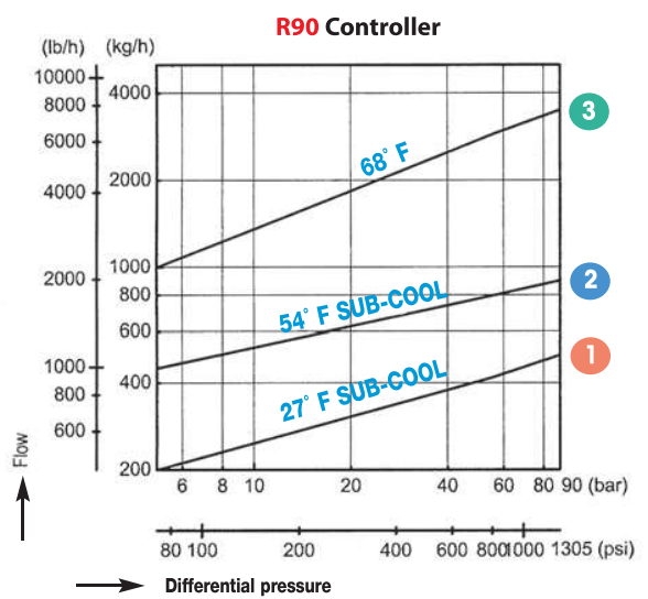
WPN-100 • 1/2", 3/4", 1"
