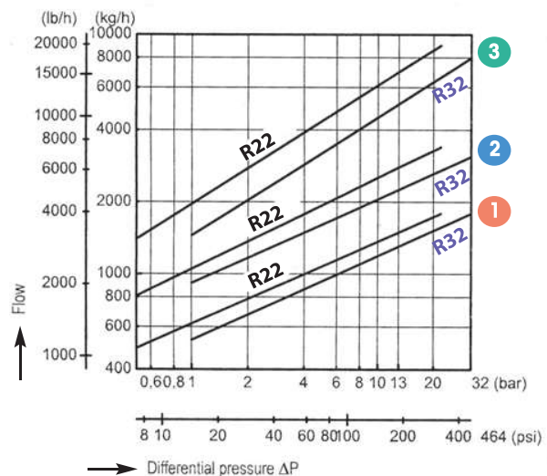
WPN-40 with R22 & R32 Controller
